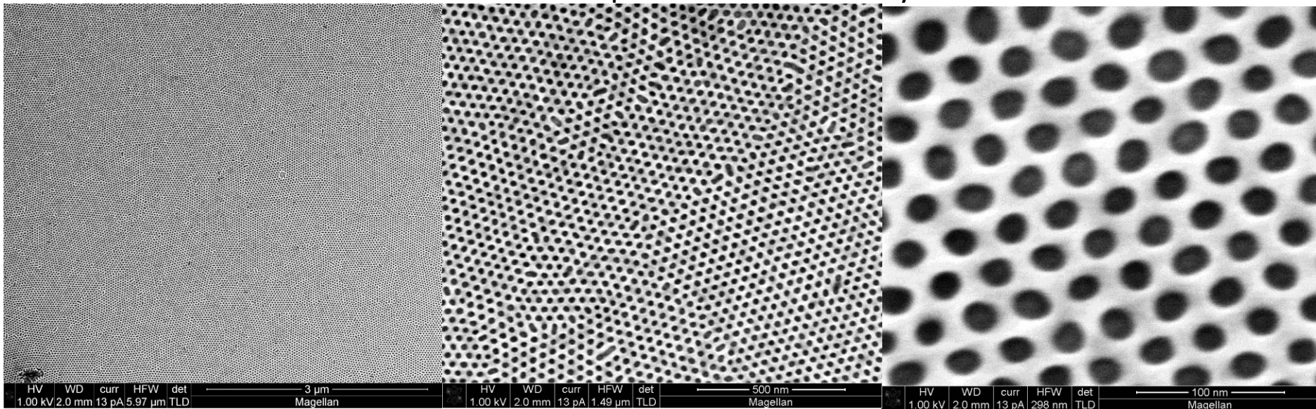
Diblock sample #2 190C 24 hr x0 y0
