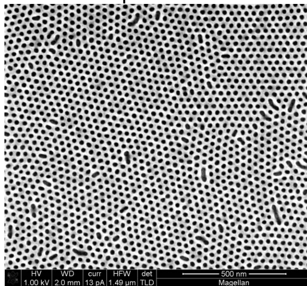
Diblock sample #1 190C 24 hr x0 y0
