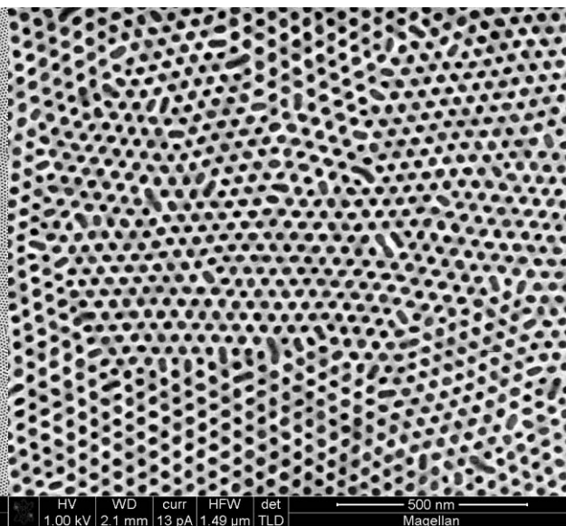
Diblock sample #1 190C 24 hr x0 y25
